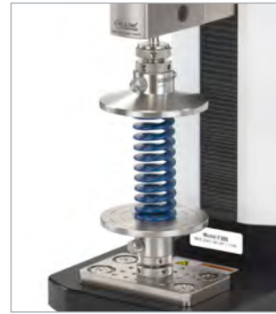
Compression spring testing
